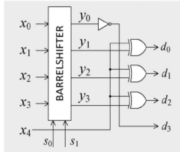
Fig 8: Address-generation circuit.
