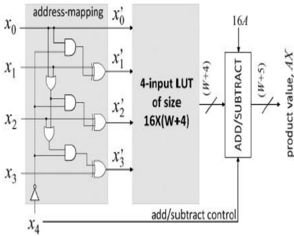
Fig. 2 LUT-based multiplier for L = 5 using the APC technique.
