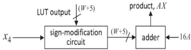
Fig.6 Modification of the add/subtract cell in Fig. 2 for the two's complement representation of product words.
