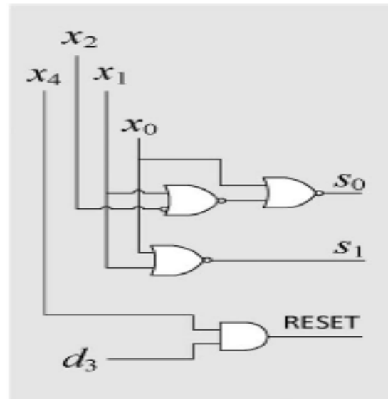
Fig.5 Control circuit for generation of s_0 , s_1 , and RESET.
