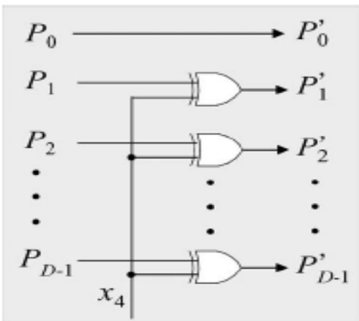
Fig7 Optimized implementation of the sign modification of the odd LUT output.
