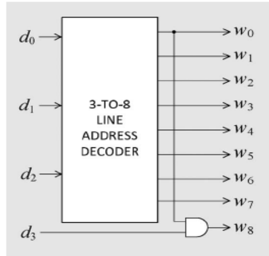
Fig. 4 Four-to-nine-line address-decoder.
