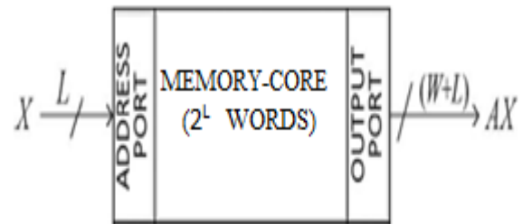
Fig.1 Conventional LUT-based multiplier.
