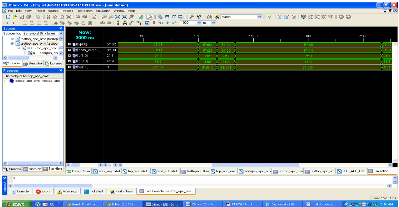
Fig 12. simulation results of top level design APC-OMS.
