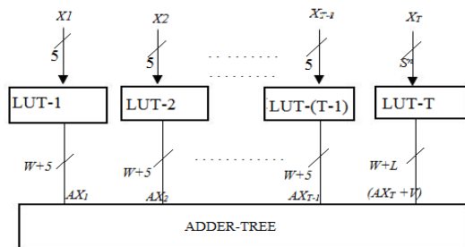
Fig.9 Proposed LUT-based multiplier for L = 5(T-1) + S' .
